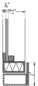
Outswing Casement
